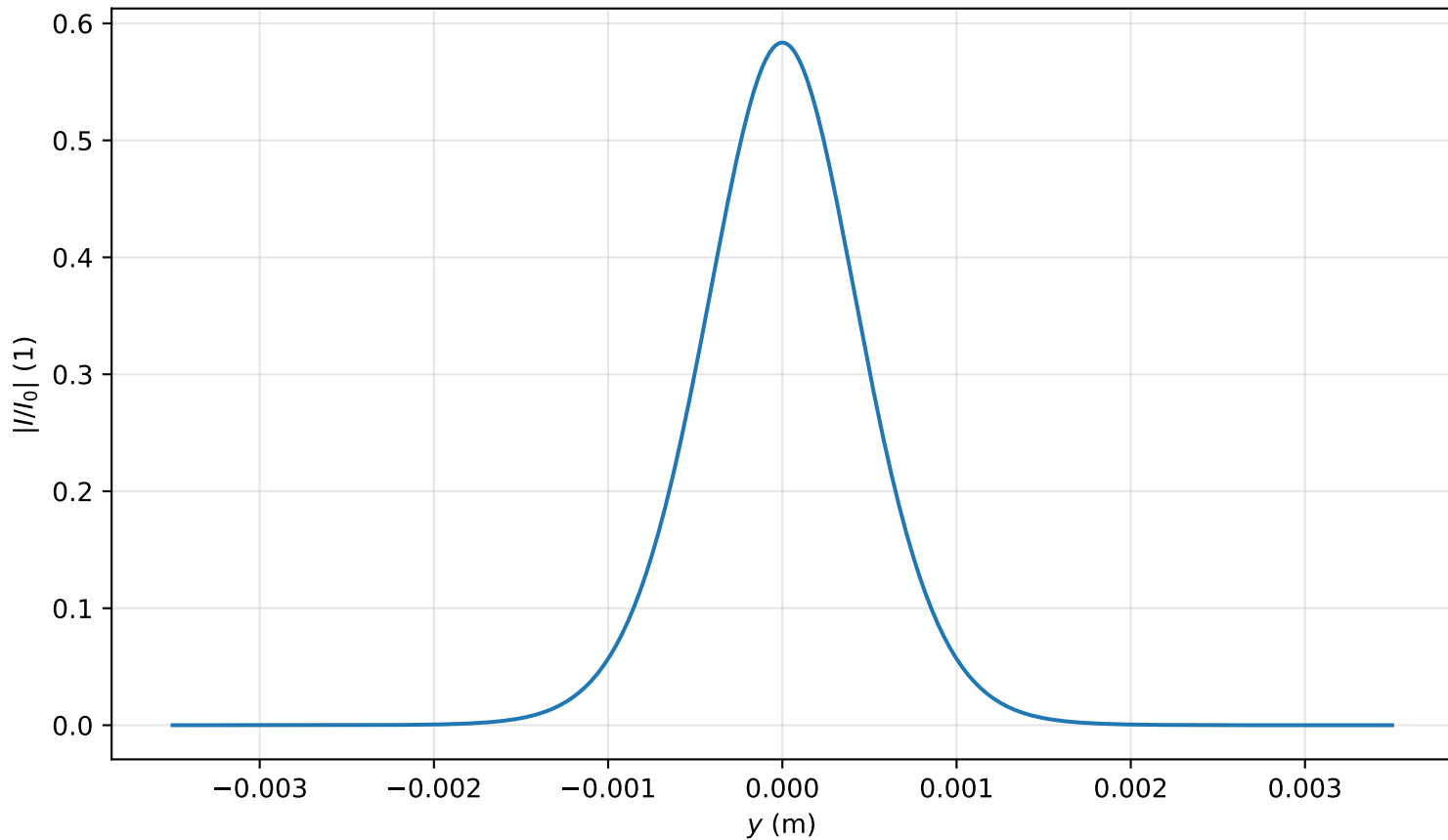
Intensity profile I(x=0, y, z=2.548)/I_0 , P_{in}=0.4P_{cr} , artificial time
